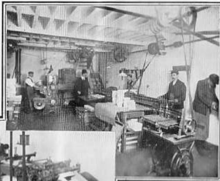
Pleated Postal Wrapper Machine.
